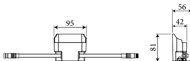
Adjustable bracket
