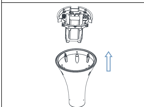
Fig.3 Take off the Plastic tray
