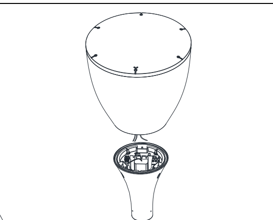
Fig.2 Take off the top part and loose the wires (LED+, LED- and GND)
