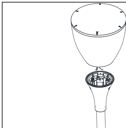
Fig.6 connect the wire (LED+,LED- and GND)
